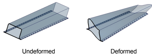
Fig. 5 Mode Shape of 1st Torsion Mode
