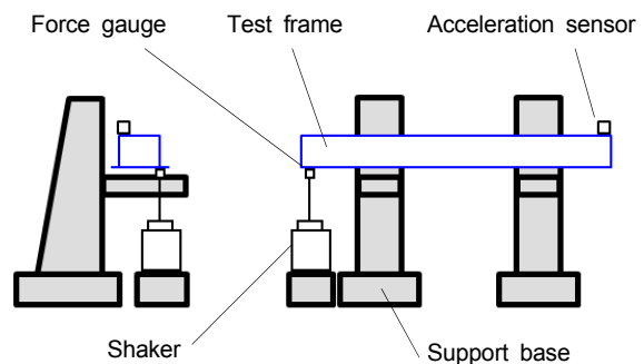
Fig. 4 Measuring System
