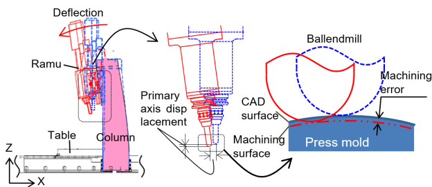
Fig. 3 Primary Axis Top End Position = Machining Error
