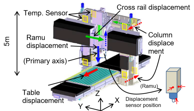
Fig. 4 Processing Machine Heat Displacement Minimization
