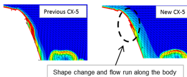
Fig. 7 Reduction of Aerodynamic Noise from A-Pillar
