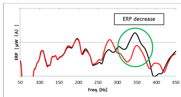
Fig. 14 Effect Confirmation of the ERP Improvement
