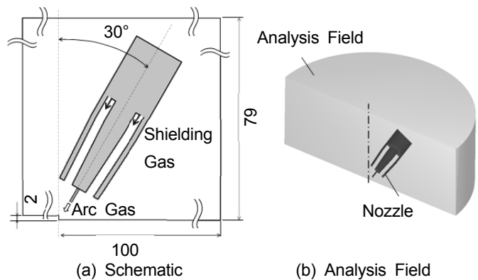
Fig. 10 Analysis Model
