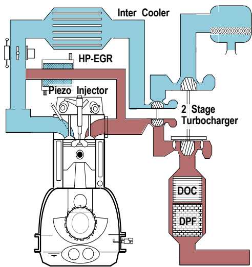
Fig. 3 Engine System
