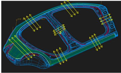
Fig. 3 Parallel Machining
