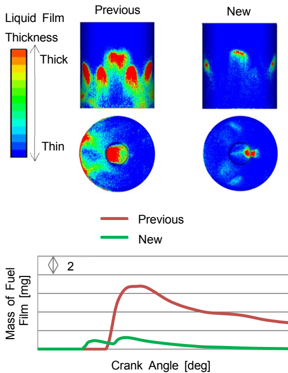
Fig. 14 Comparison of Fuel Film at Light Load
