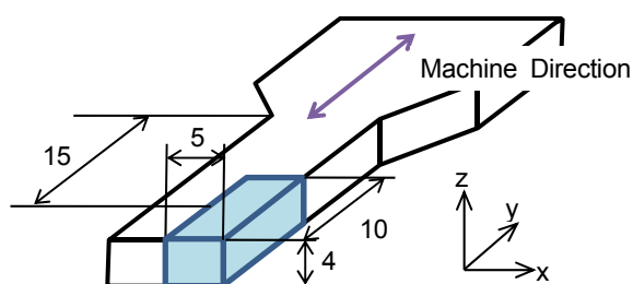
Fig. 1 Measured Part for Fiber Orientation
