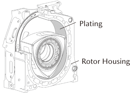
Fig. 16 Trochoid Plating
