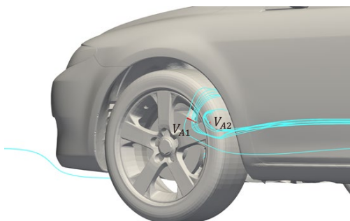
Fig. 9 Streamlines Passing through Vortices V_{A1} and V_{A2}
