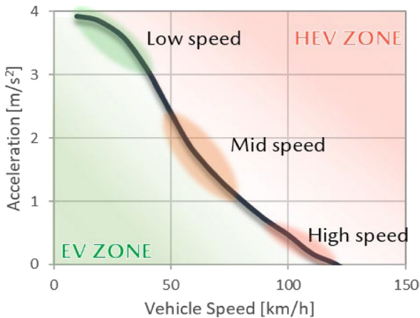
Fig. 7 Engine Operating Line for Vehicle Speed and Acceleration
