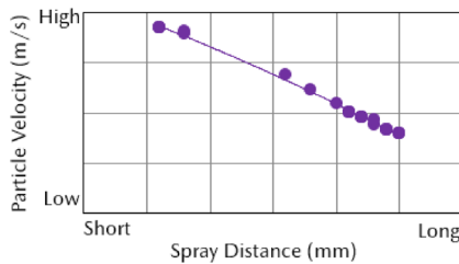
Fig. 10 Effect of Spray Distance on Particle Velocity
