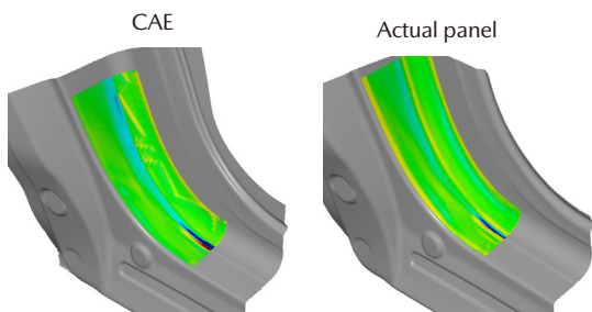
Fig. 12 Mold Modification Process Application Results
