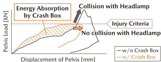
Fig. 19 Energy Absorption Performance and Pelvis Load
