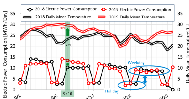
Fig. 10 Changes in Daily Electric Power Consumption and Mean Temperature of Office Building Air Conditioning Equipment in September 2018 and 2019
