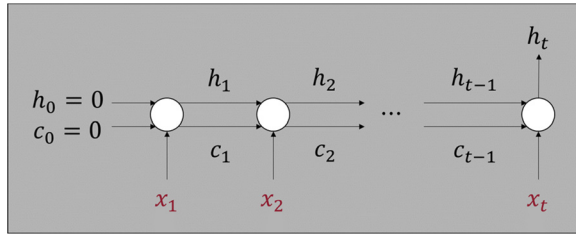
Fig. 4 Structure of LSTM
