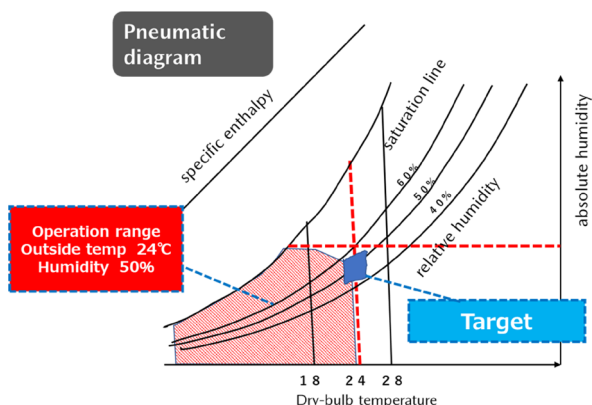
Fig. 8 Psychrometric Chart
