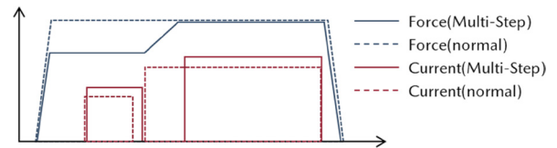
Fig. 27 Welding Condition
