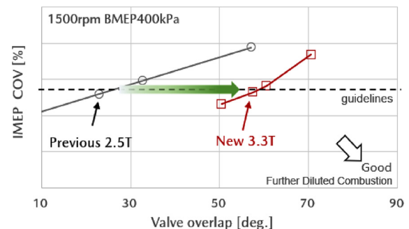
Fig. 11 Valve Overlap and IMEP Coefficient of Variation
