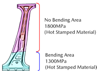
Fig. 9 B-pillar Material
