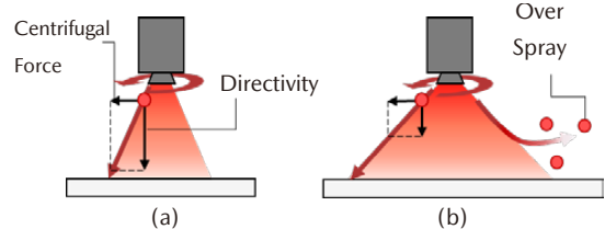
Fig. 16 Spray Pattern
