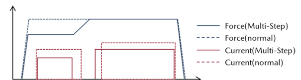
Fig. 28 Welding Condition
