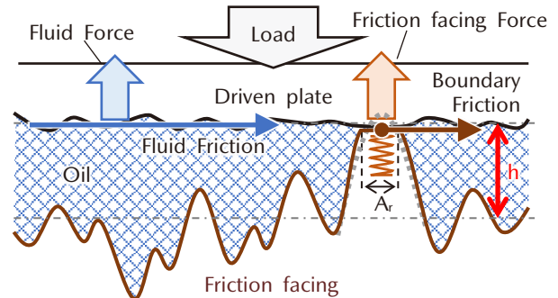
Fig. 9 Conceptual Diagram of Friction Facing Surface
