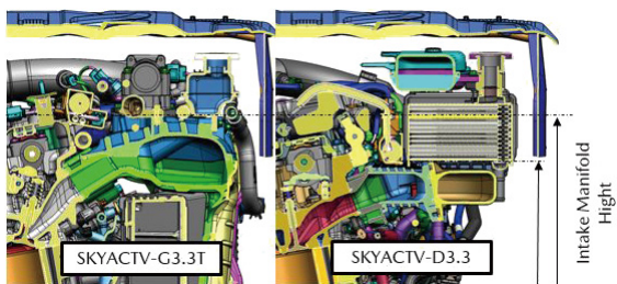
Fig. 5 Cross-Sectional Diagram of Intake Manifold
