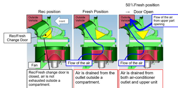
Fig. 13 Operation Explanation of Blower Unit.
