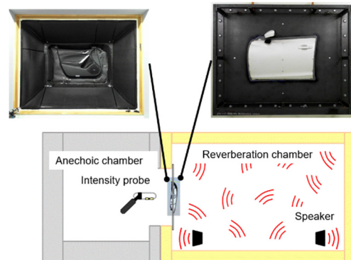
Fig. 9 Reverberation Anechoic Chamber
