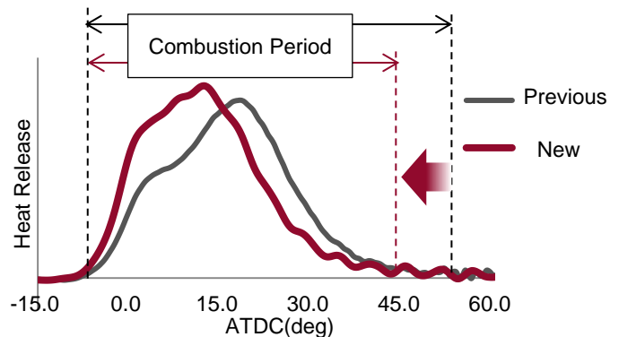
Fig. 7 Heat Release
