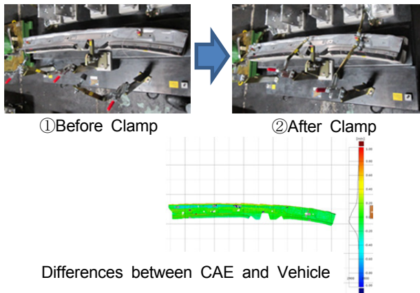
Fig. 8 Clamp Simulation
