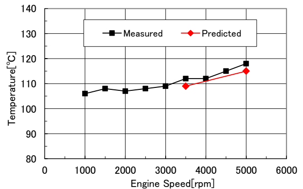
Fig. 10 Comparison of Crank-Pin Bearing Temperature
