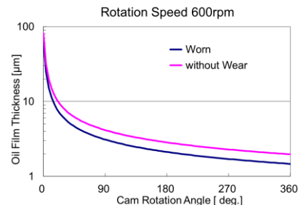
Fig. 13 Camshaft Thrust Bearing Oil Film Thickness
