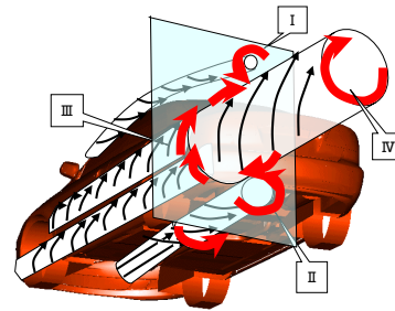
Fig. 1 Flow Structure around a Vehicle 2)
