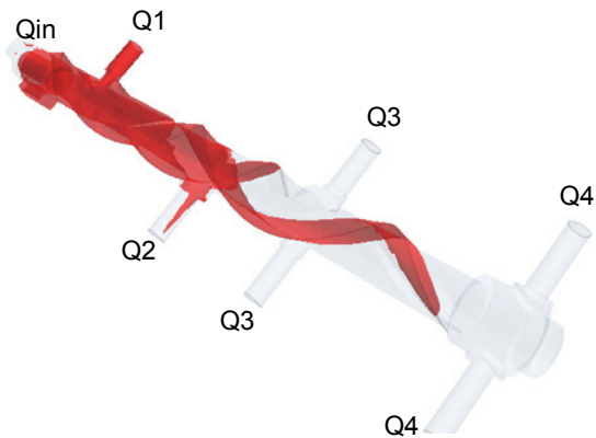
(b) Fluid Analysis Fig. 9 Oil Flow in Oil Pipe by CAE
