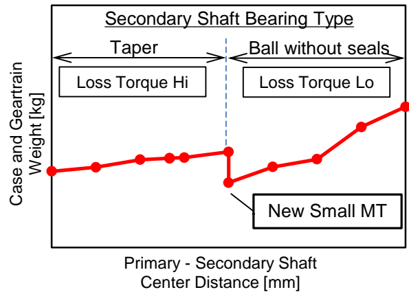
Fig. 3 Relation between Center Distance and Weight
