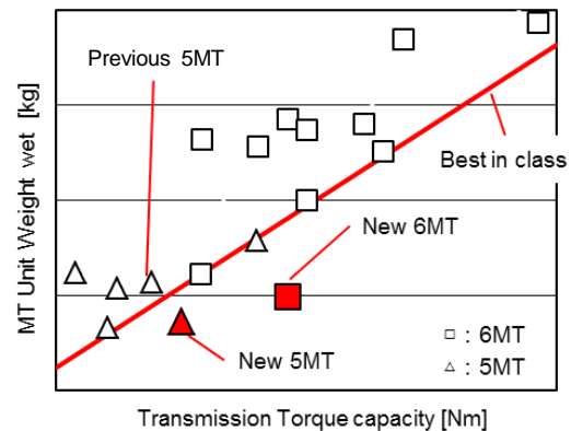
Fig. 4 Transmission Weight
