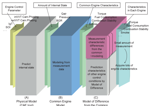
Fig.15 Approach of Engine Modeling
