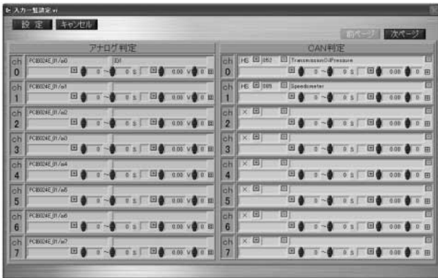
Fig.14 Error Detection Setting
