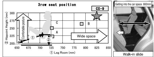
Fig.4 3 rd Row Seat Position and Walk-in Space
