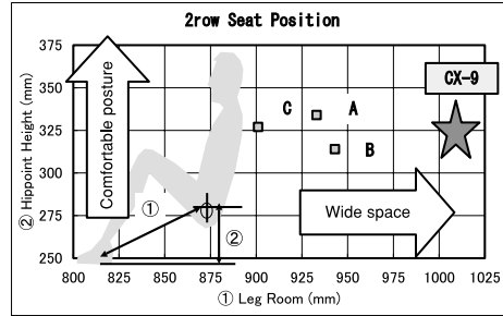
Fig.3 2 nd Row Seat Position
