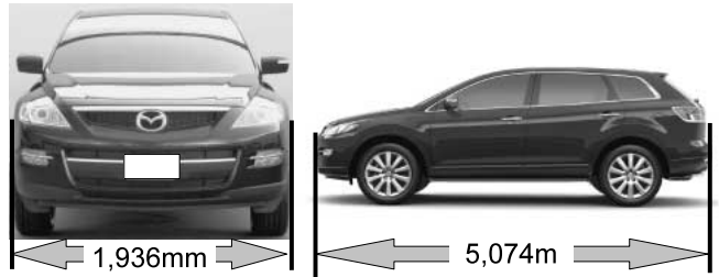
Fig.1 Exterior Dimensions
