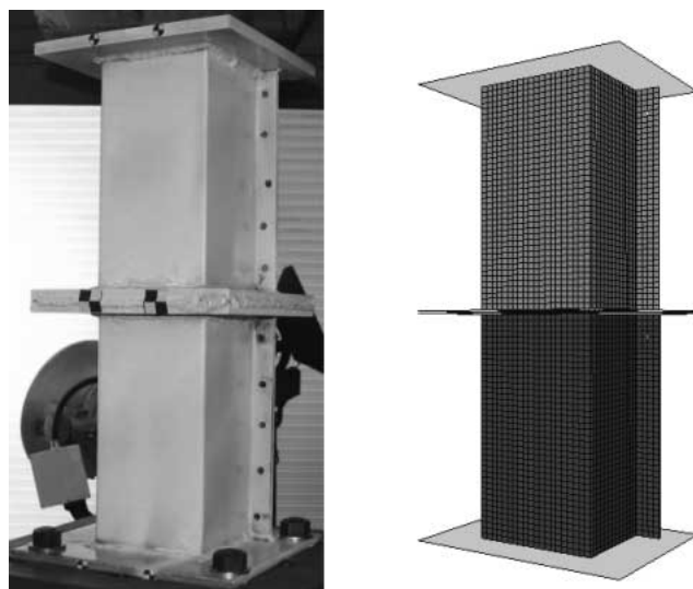
Fig.5 Drop Weight Test with Two Test Pieces Piled Up
