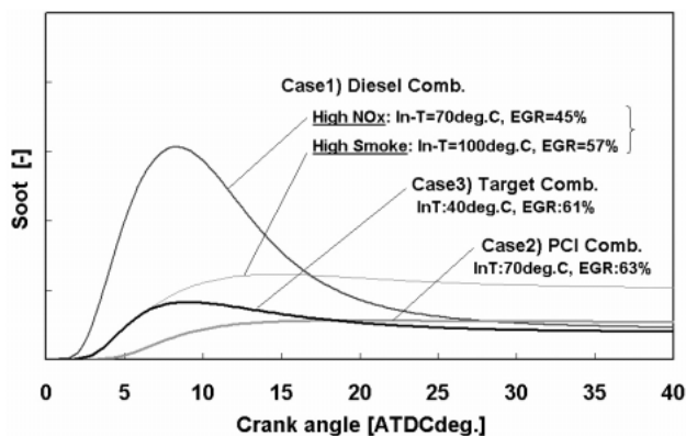
Fig.4 Comparison of Soot Amount History
