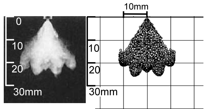
(b) Spray Image t = 1.5\text{ms} (ASOI)
