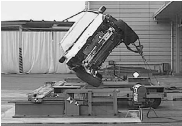
Fig.14 Trip Over Test
