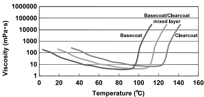
Fig.2 Ideal Curing Behavior of Top Coat Paint
