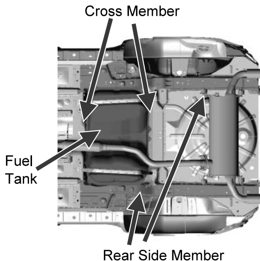
Fig.17 Rear Impact Structure
