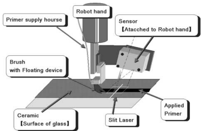
Fig.12 Attachment of a Sensor to a Primer Application Robot Hand
