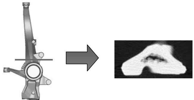
Fig.3 Shrinkage Form Section & CT Scanner Image
