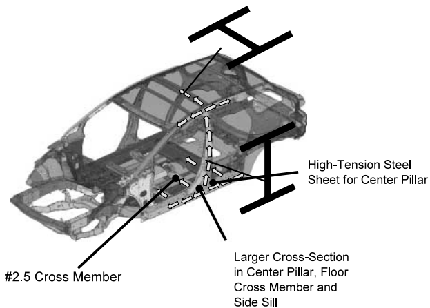
Fig.16 Side Impact Structure
