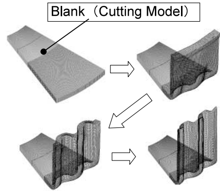
Fig.6 Clutch Hub Spline Forming Simulation
