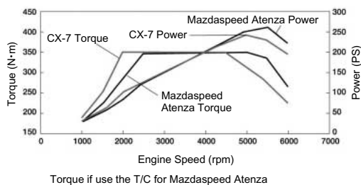
Fig.11 Engine Performance
