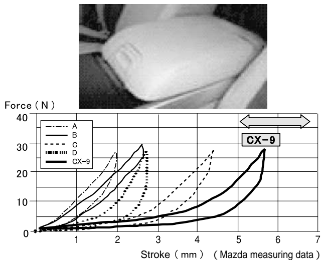
Fig.6 Deflection Variance of Armrest Cushion
