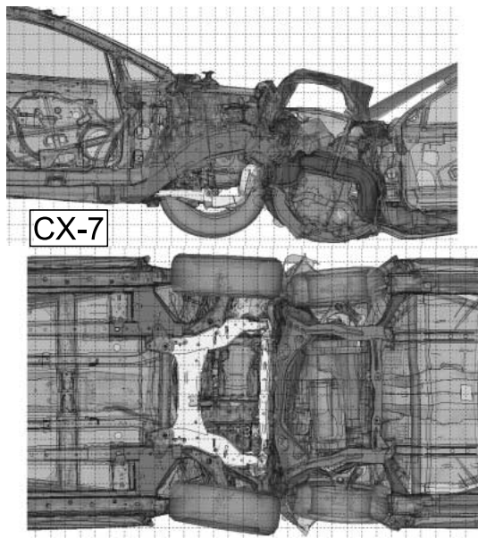
Fig.15 Compatibility CAE
