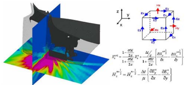
Fig.8 FDTD Analysis
